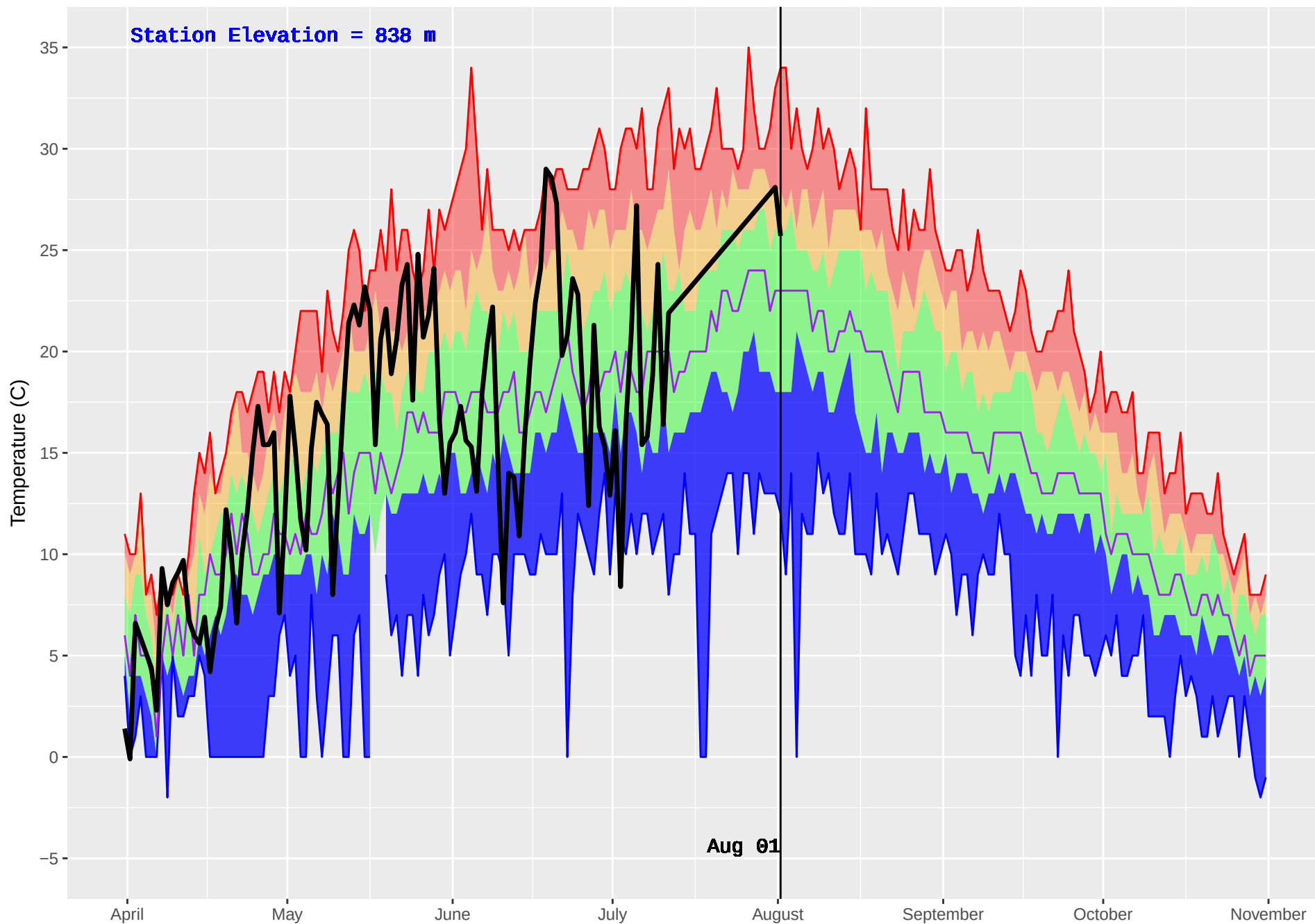
HOWARD (343) : Historical (1970–2016) and Current (2018) Daily Temperature
