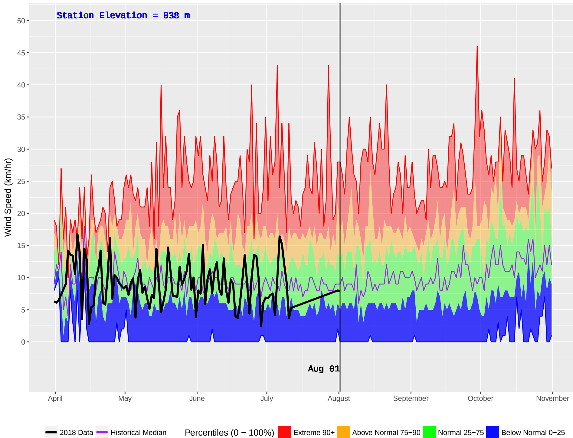
HOWARD (343) : Historical (1970–2016) and Current (2018) Daily Wind Speed
