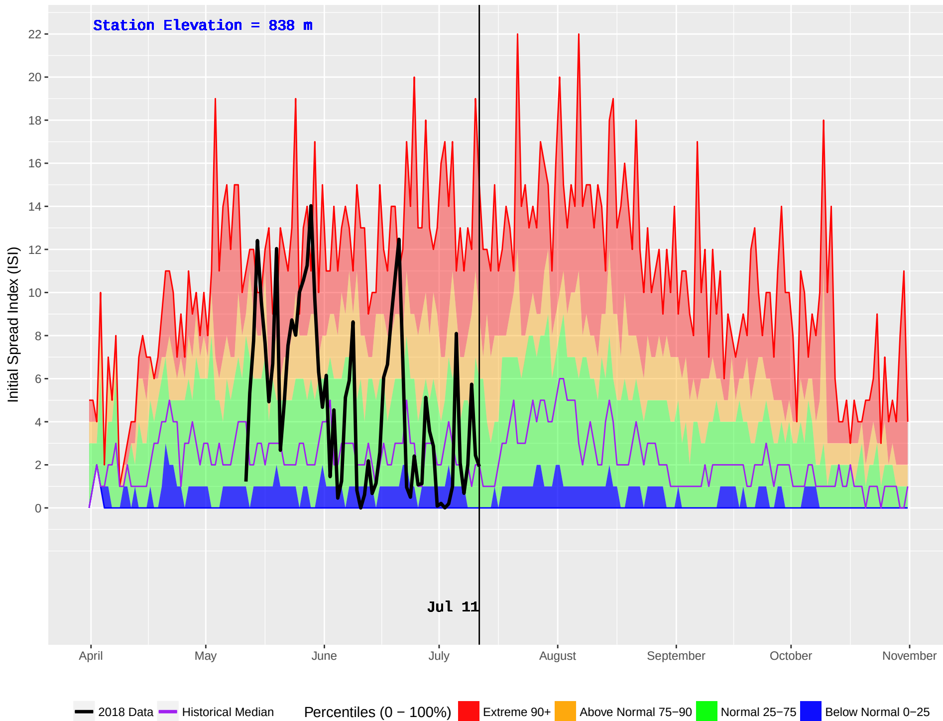
HOWARD (343) : Historical (1970–2016) and Current (2018) Daily Initial Spread Index (ISI)
