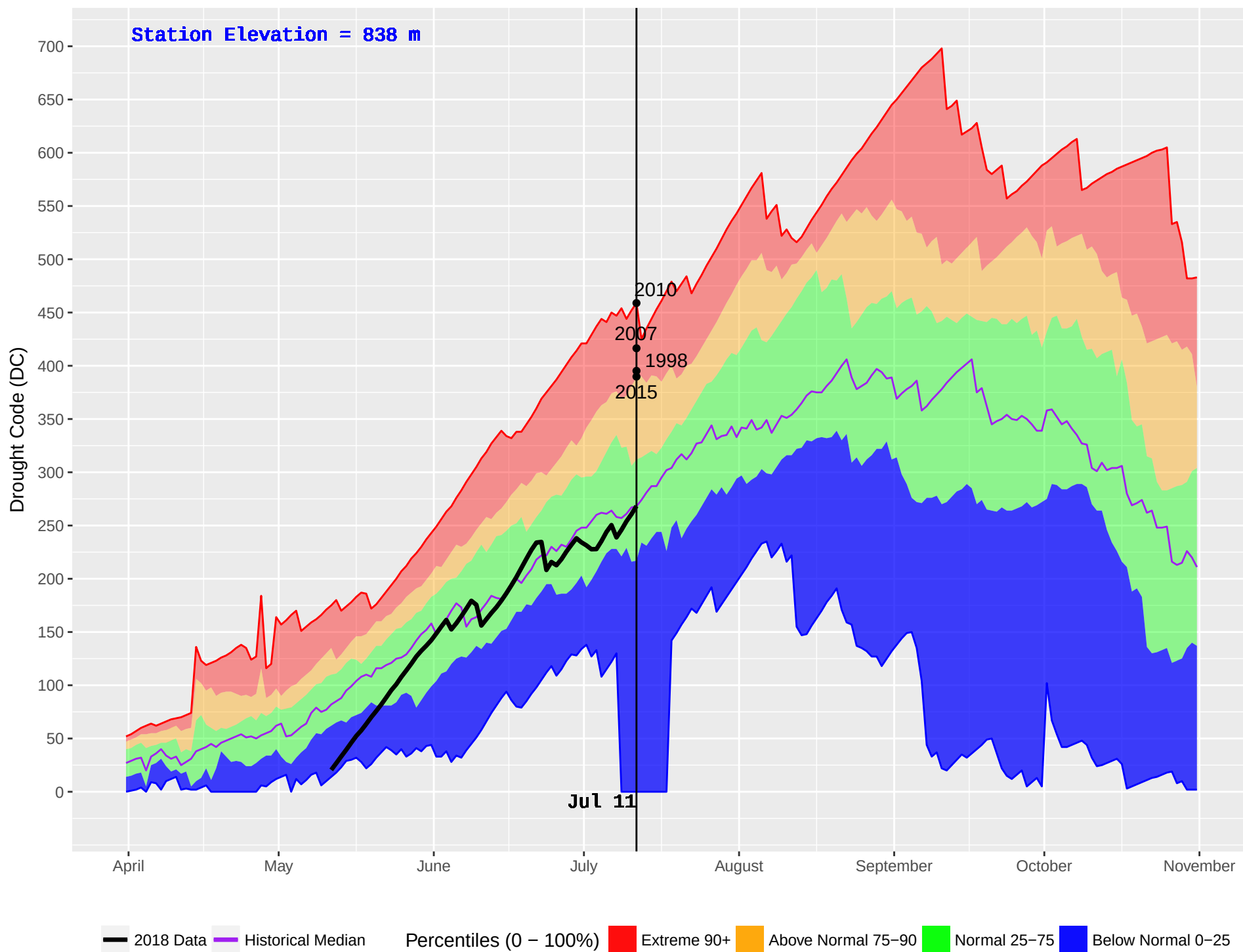
HOWARD (343) : Historical (1970–2016) and Current (2018) Daily Drought Code (DC)
