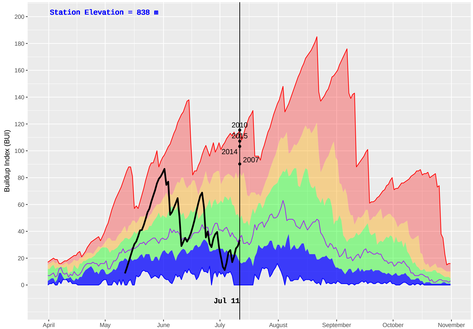
HOWARD (343) : Historical (1970–2016) and Current (2018) Daily Buildup Index (BUI)
